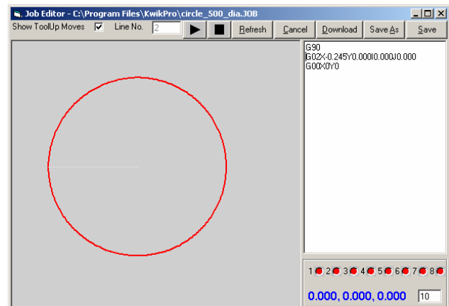
Simple G Code program defining the path.
